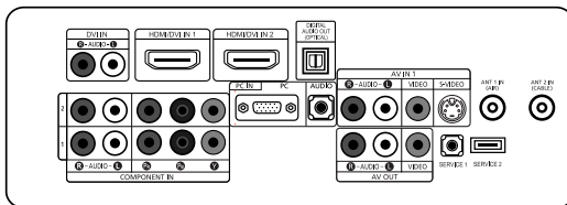
JACK PANEL DETAIL 3.25" H x 9.92" W @ 12.98" UP FROM BOTTOM
